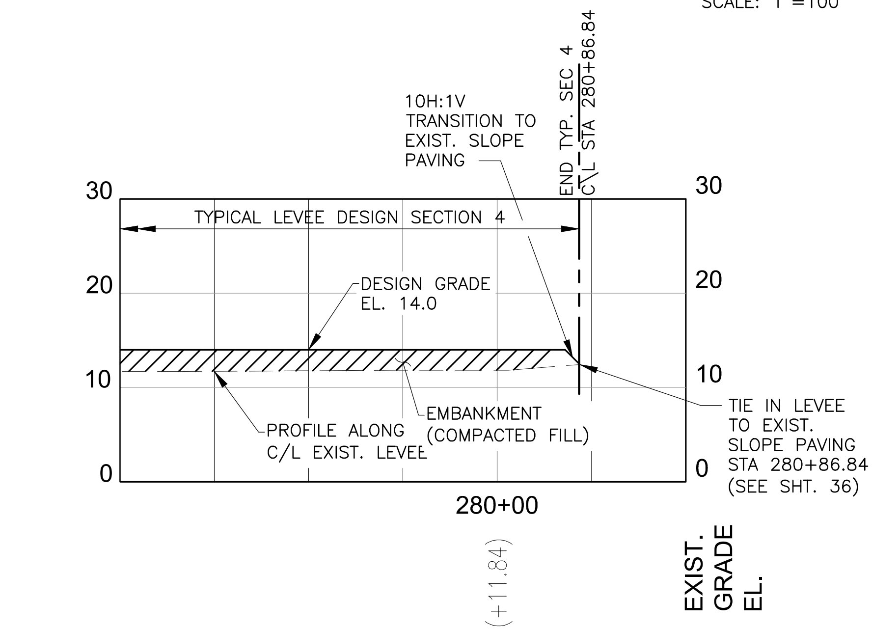
PROFILE
