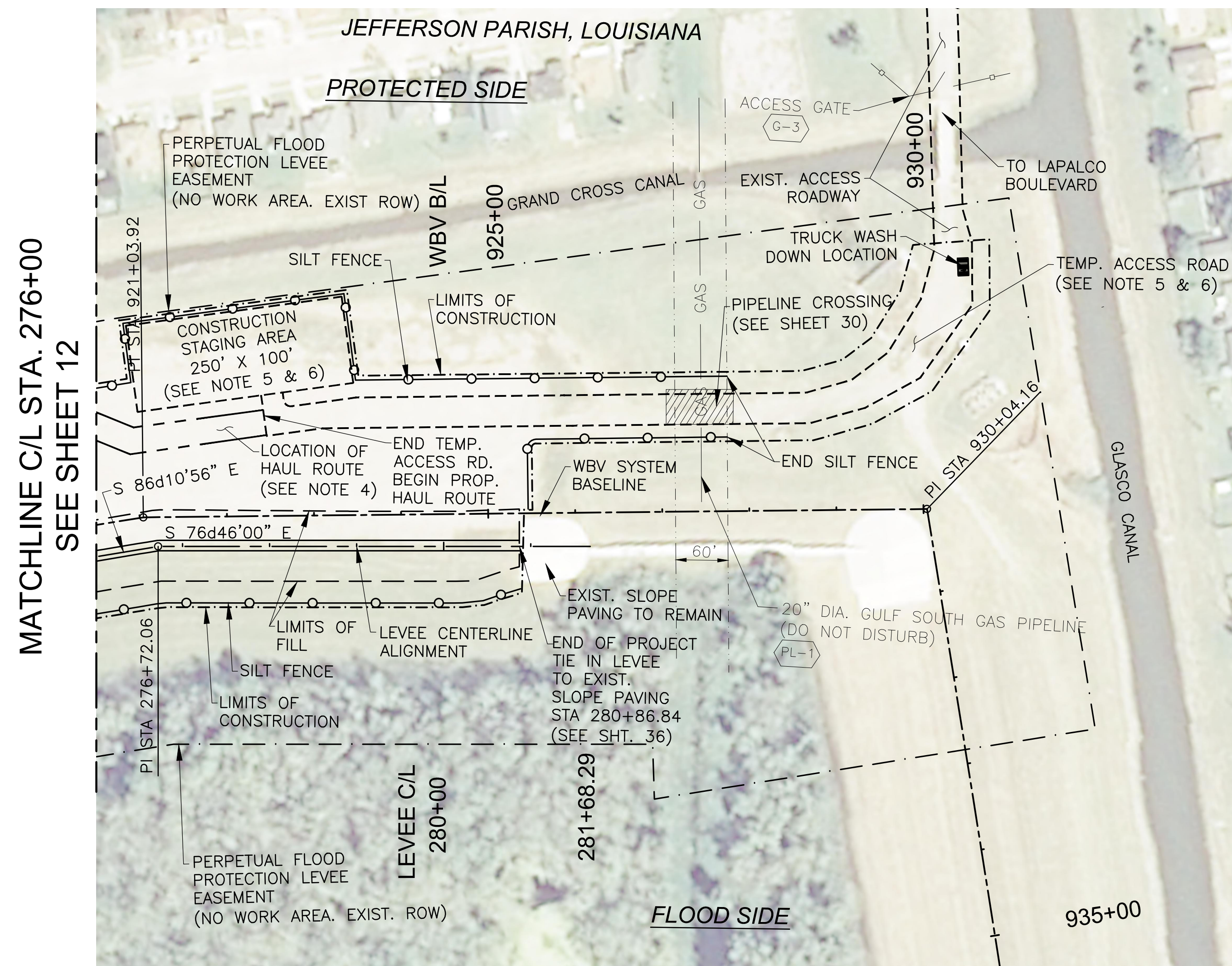
PLAN
