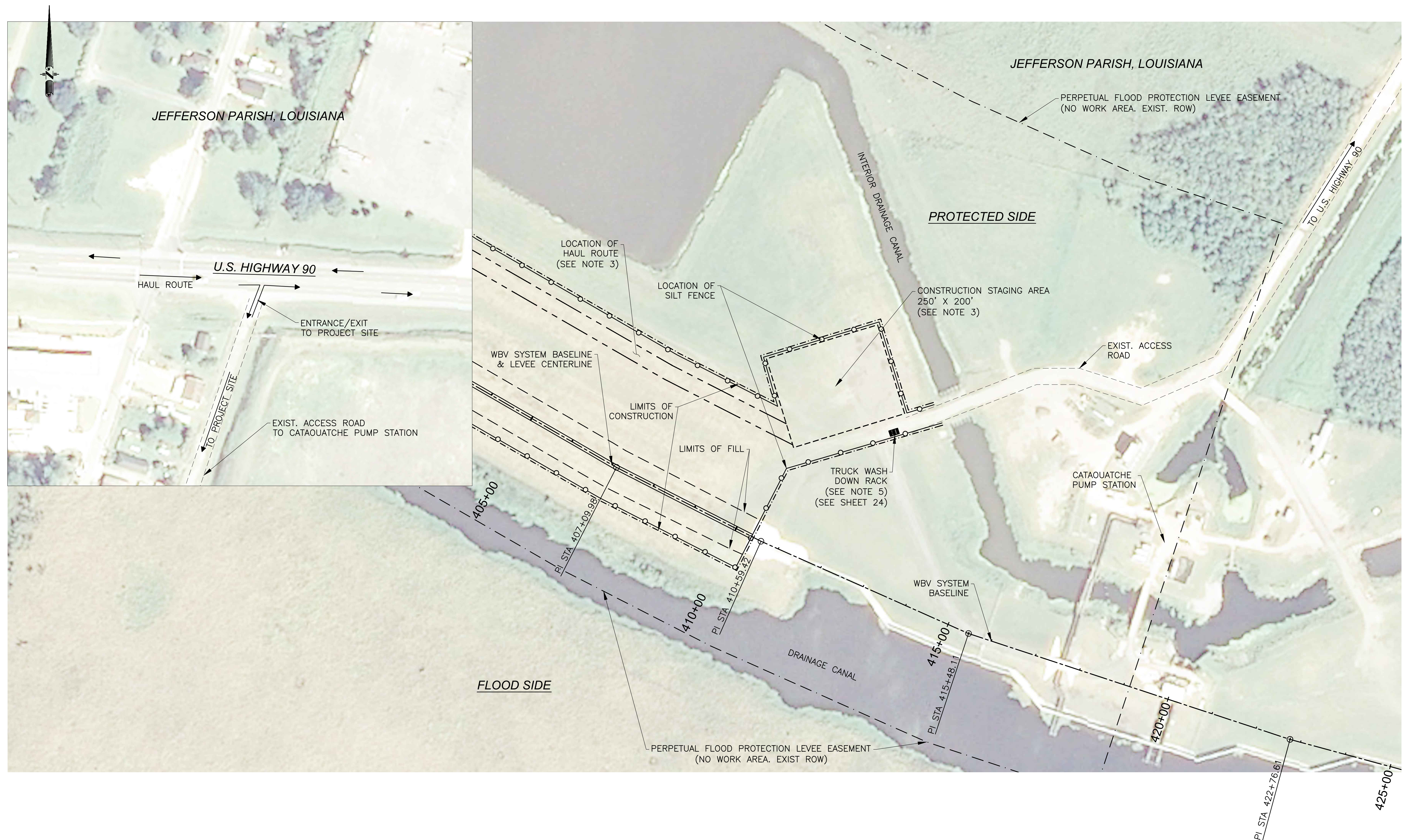
CONSTRUCTION ACCESS PLAN
